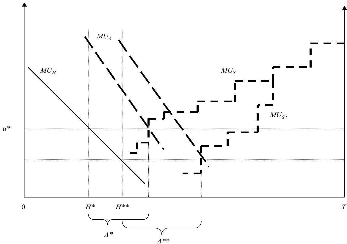
Figure 1 The Implications of Fewer Current Contacts
